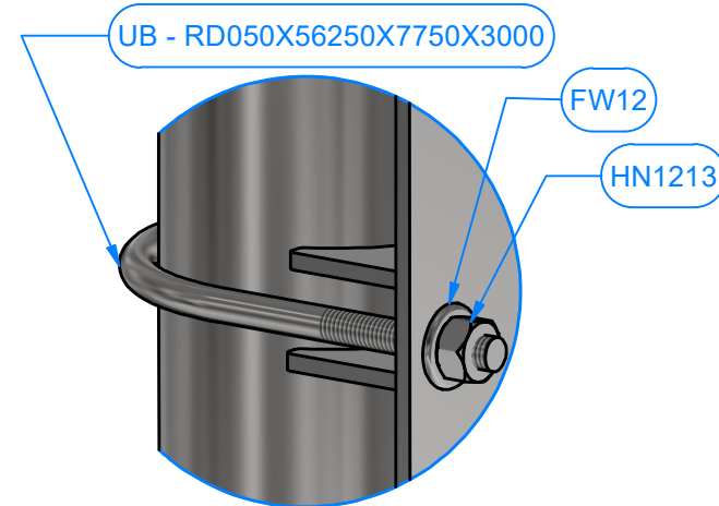
DETAIL D
