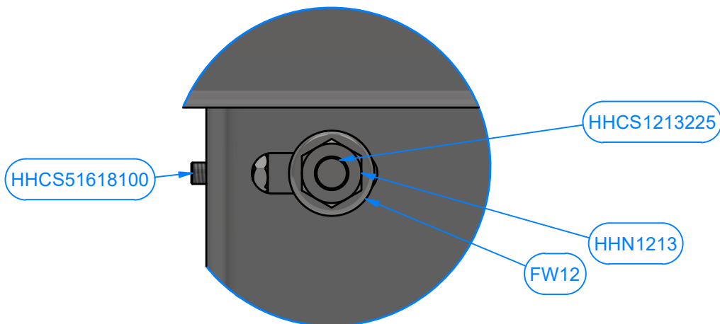
DETAIL F
