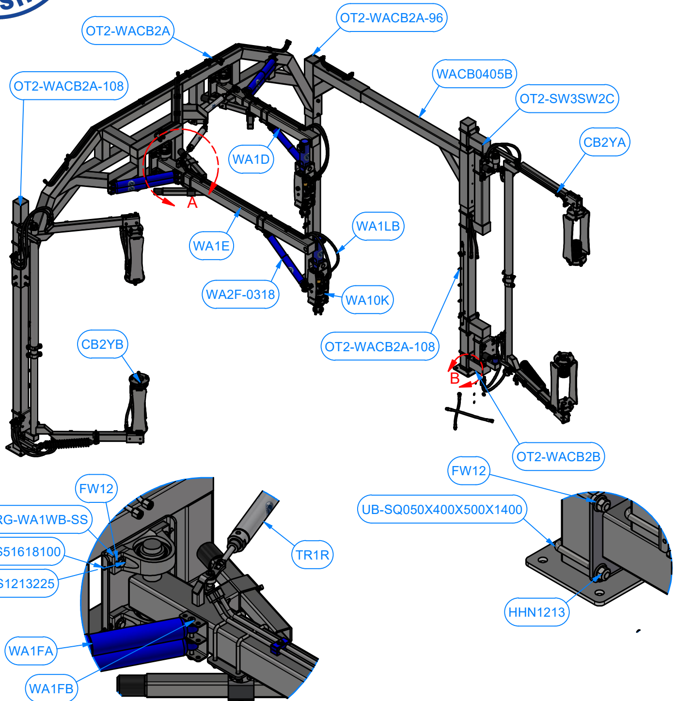
DETAIL B
