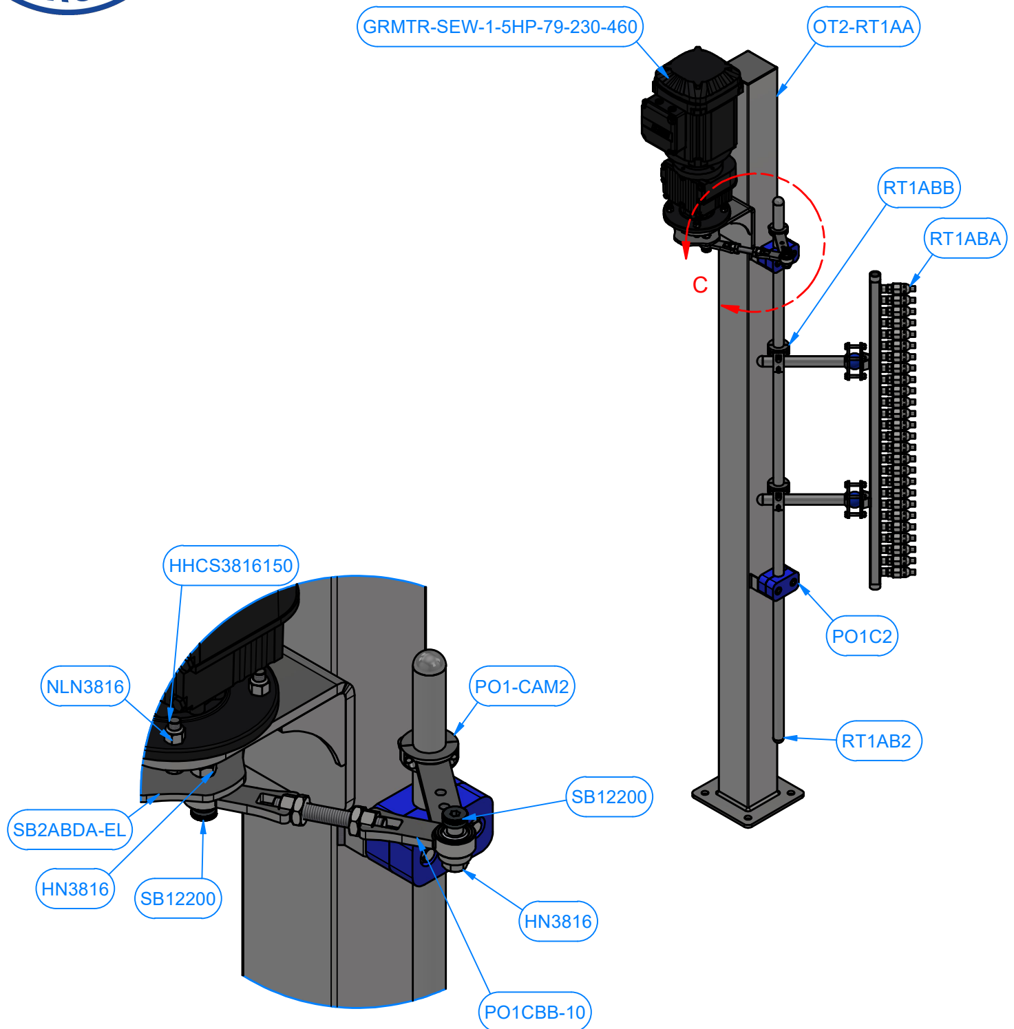
DETAIL C
