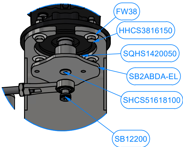
DETAIL F
