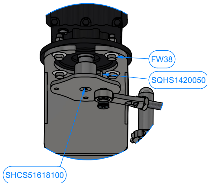
DETAIL D
