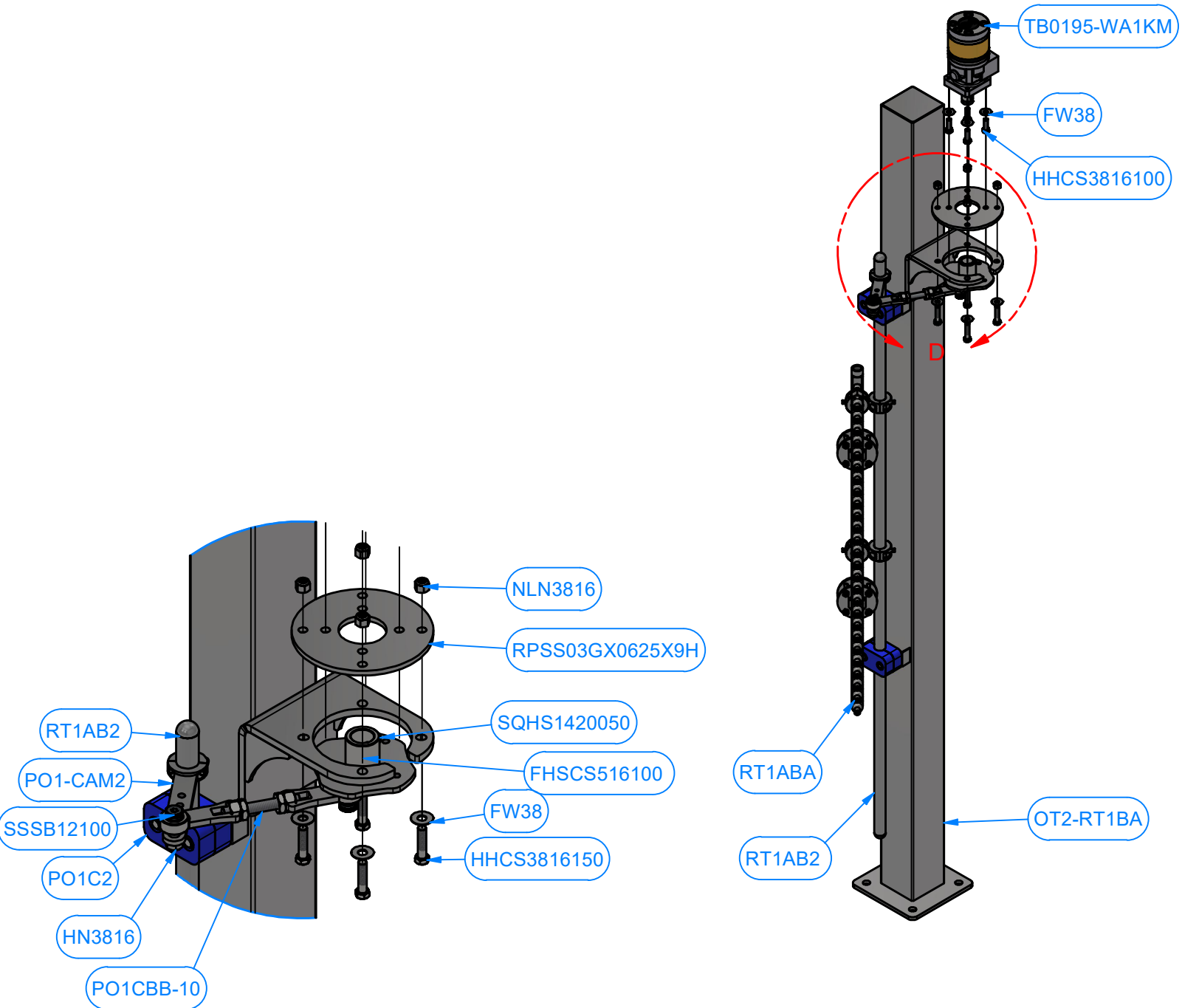
DETAIL D
