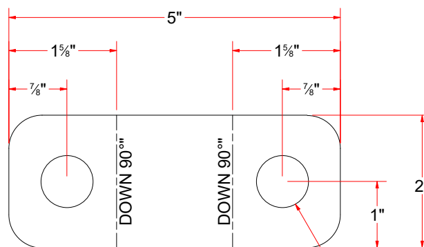
FLAT PATTERN
