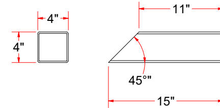
Sq. Tube 4" x Wall x 15" LG.
