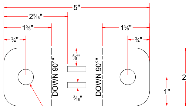
FLAT PATTERN
