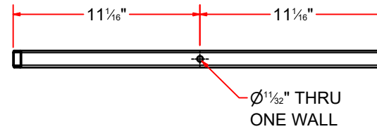
Sq.Tubing 1" x 22 1/16" LG.
