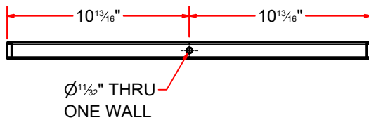
Sq.Tubing 1" x 21 5/8" LG.
