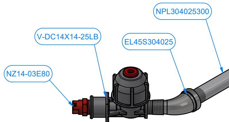
DETAIL U
