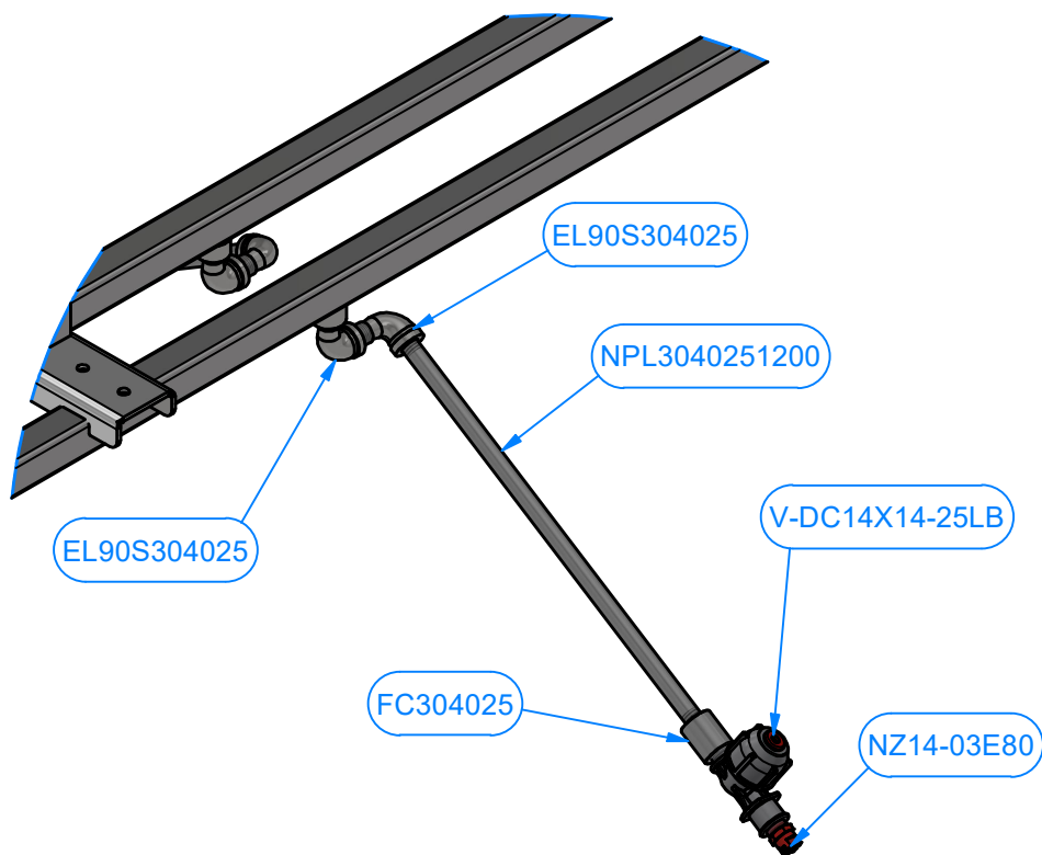
DETAIL T
