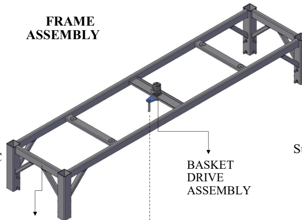
2. FRAME
