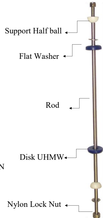
BASKET DRIVE ASSEMBLY
