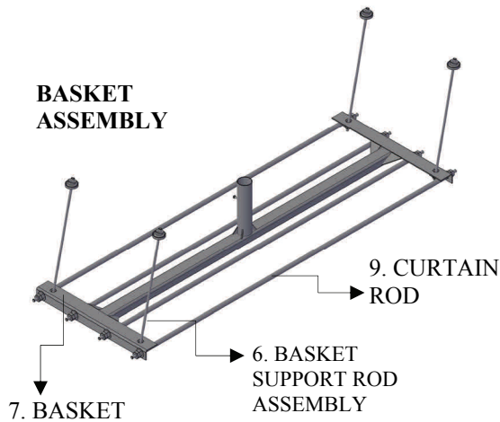
6. BASKET SUPPORT ROD ASSEMBLY
