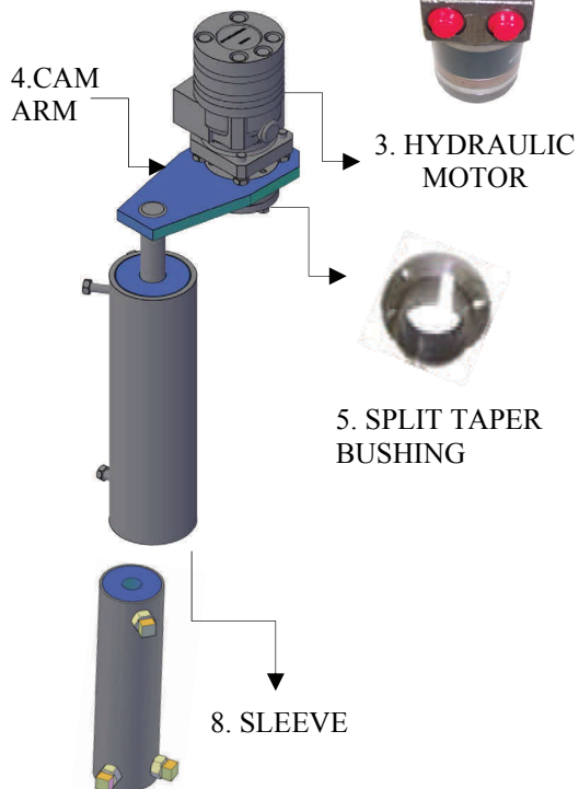
BASKET DRIVE ASSEMBLY
