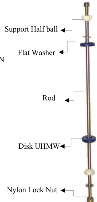
6. BASKET SUPPORT ROD ASSEMBLY
