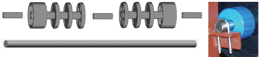
UHMW SUPPORT ROLLER for BELT w/PUSHERS w/ROUND U BOLTS and SHAFT 3/4" and UHMW SPACERS 3/4" I.D.
