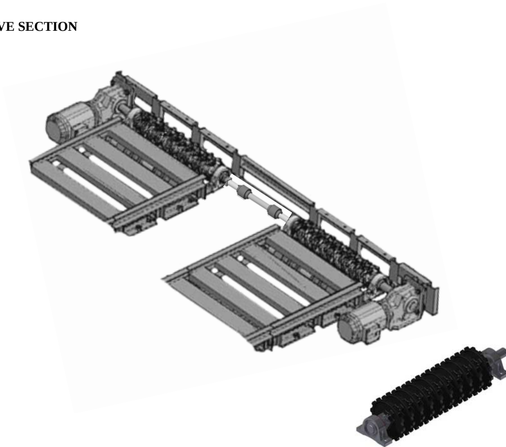
DRIVE SHAFT w/PILLOW BLOCKS and PASTIC SPROCKETS
