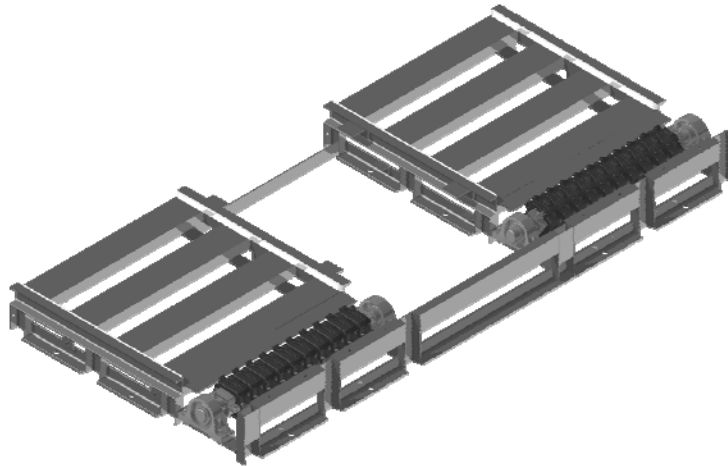
BELT w/o PUSHERS
