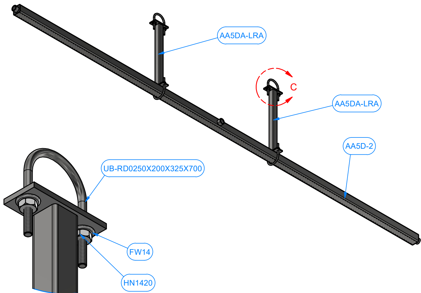
DETAIL C SCALE 3:5
