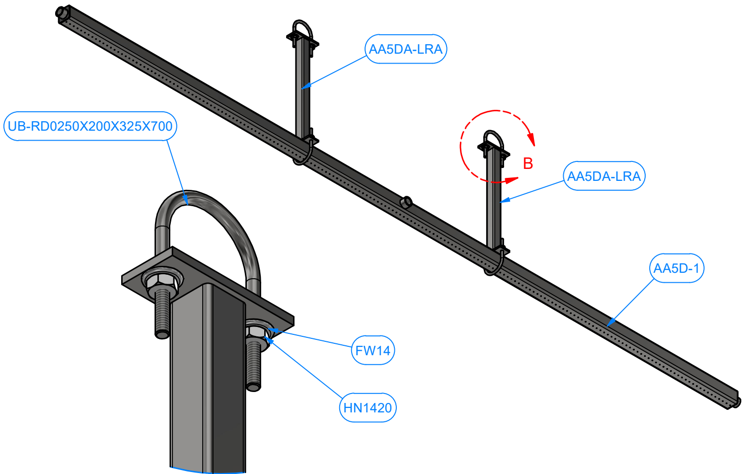
DETAIL B SCALE 3:5
